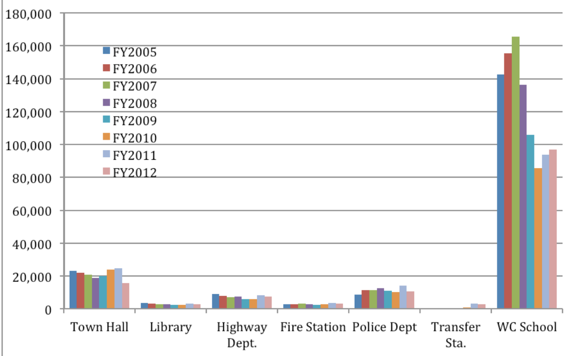
Warwick town buildings - Electricity used each year in kWhrs
